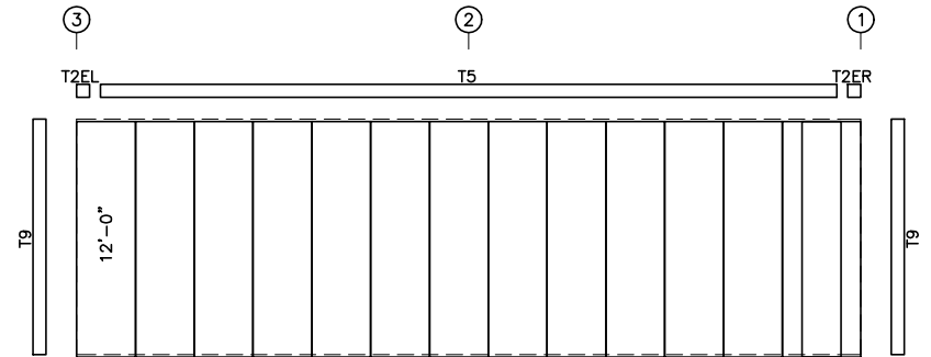
SIDEWALL SHEETING & TRIM: FRAME LINE C PANELS: 26 Ga. 6PBR - Sil Poly
