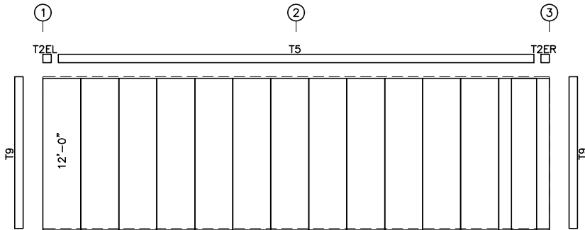
SIDEWALL SHEETING & TRIM: FRAME LINE A PANELS: 26 Ga. 6PBR - Sil Poly
