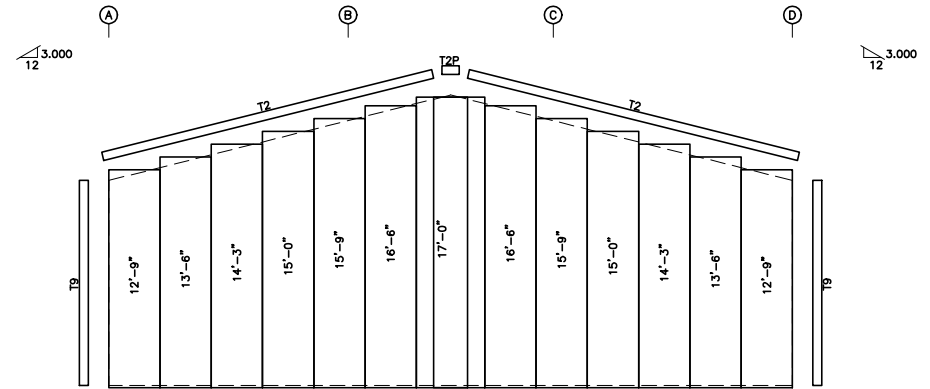
ENDWALL SHEETING & TRIM: FRAME LINE 4 PANELS: 26 Ga. 6PBR - SII Poly
