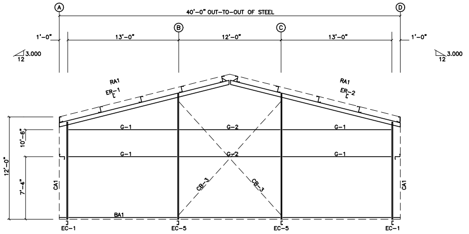
ENDWALL FRAMING: FRAME LINE 4
